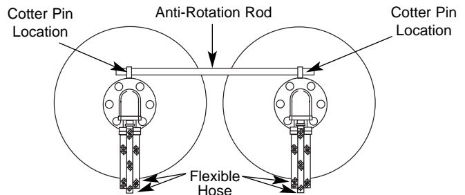
Horizontal installation of rod in body lugs.
