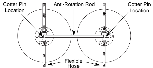
Horizontal installation of rod in head lugs.
